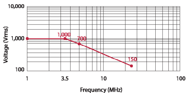
Figure 2 Derating Curve
