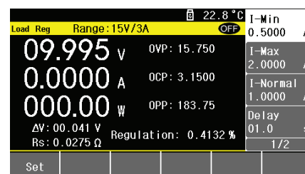
Load regulation test
