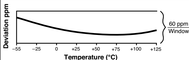
Figure 1 – A Typical VHP10x Resistance Temperature Curve
