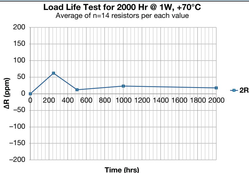
FIGURE 5 - LOAD LIFE TEST
