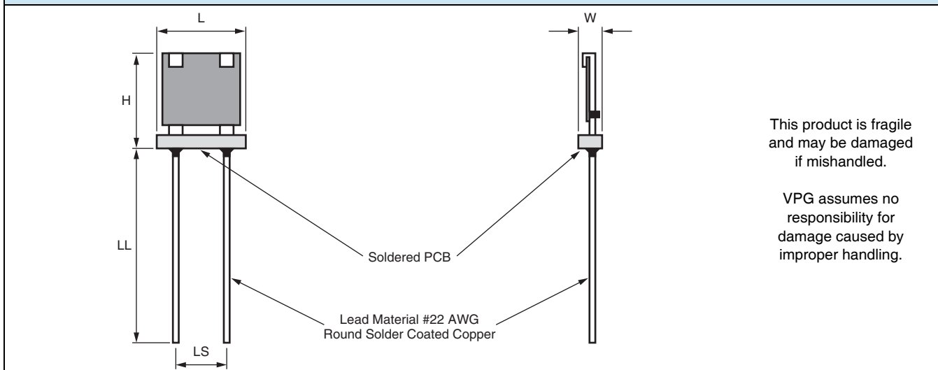
FIGURE 2 - STANDARD DIMENSIONS
