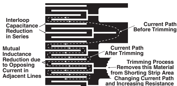
FIGURE 3 - TRIMMING TO VALUES (conceptual illustration)
