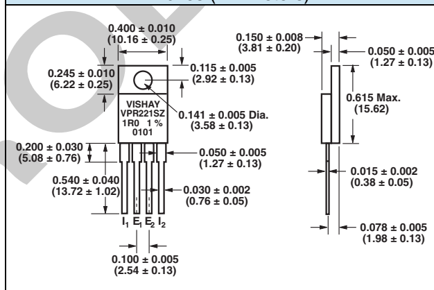
FIGURE 6 - VPR221SZ DIMENSIONS in inches (millimeters)
