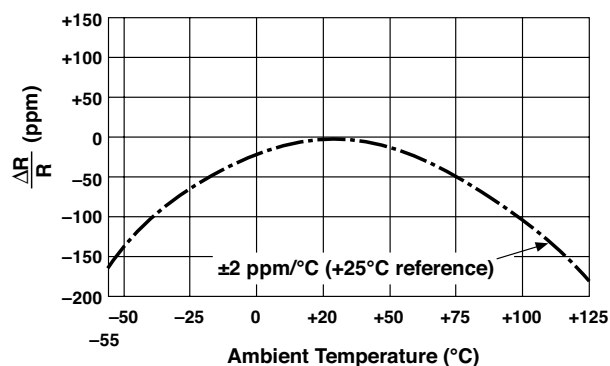
Figure 4 – Typical TCR Curve (for more details, see Table 2)
