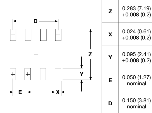
Figure 6 – Land Pattern in inches (millimeters)
