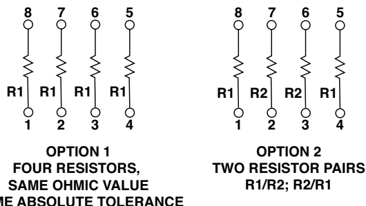
Figure 1 – Schematics (1)
