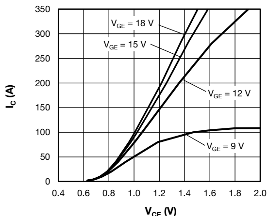
Fig. 4 - Typical Output Characteristics vs. V_{GE} at 125^\circ\text{C}
