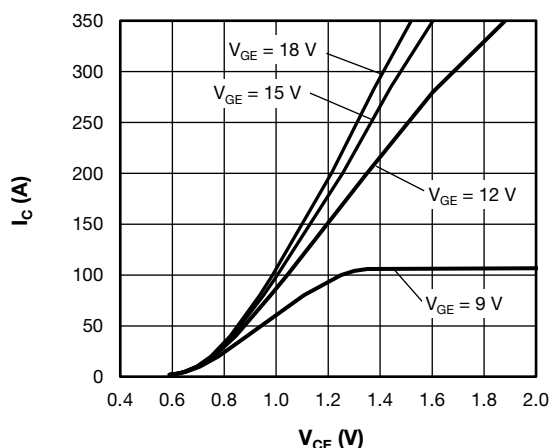
Fig. 5 - Typical Output Characteristics vs. V_{GE} at 150^\circ\text{C}
