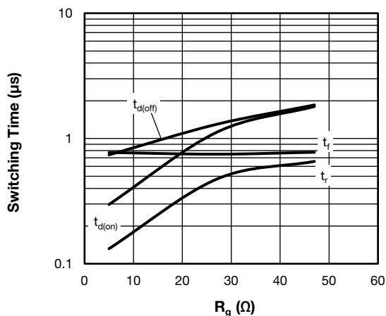
Fig. 12 - Typical IGBT Switching Time vs. R_g T_J = 125^\circ\text{C} , I_C = 200\text{ A} , V_{CC} = 480\text{ V} , V_{GE} = 15\text{ V} , L = 500\text{ }\mu\text{H} , R_g = 5\text{ }\Omega , Diode used: 60APH06
