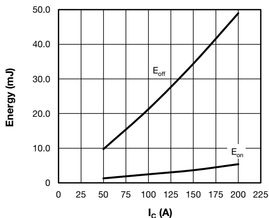
Fig. 9 - Typical IGBT Energy Losses vs. I_C T_J = 125^\circ\text{C} , V_{CC} = 480\text{ V} , V_{GE} = 15\text{ V} , L = 500\text{ }\mu\text{H} , R_g = 5\text{ }\Omega Diode used: 60APH06
