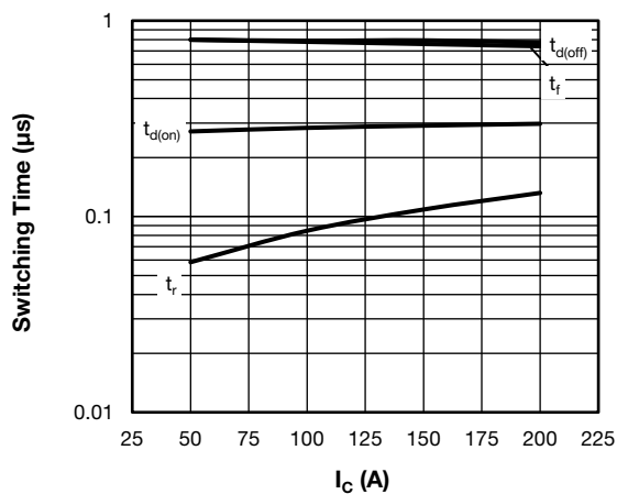
Fig. 10 - Typical IGBT Switching Time vs. I_C T_J = 125^\circ\text{C} , V_{CC} = 480\text{ V} , V_{GE} = 15\text{ V} , L = 500\text{ }\mu\text{H} , R_g = 5\text{ }\Omega Diode used: 60APH06
