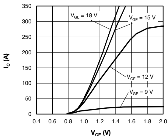
Fig. 3 - Typical Output Characteristics vs. V_{GE} at 25^\circ\text{C}
