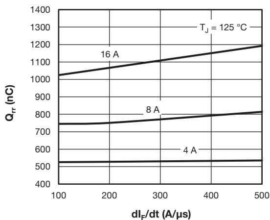
Fig. 11 - Typical Stored Charge vs. dl_F/dt
