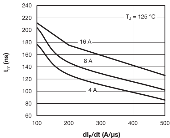
Fig. 9 - Typical Reverse Recovery Time vs. dl_F/dt
