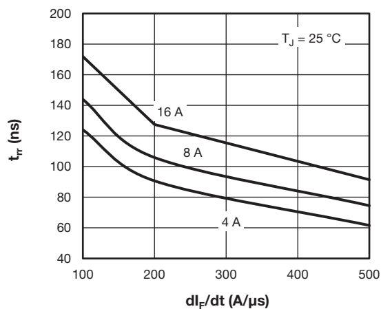
Fig. 8 - Typical Reverse Recovery Time vs. dl_F/dt
