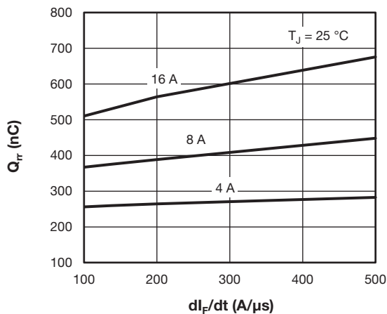
Fig. 10 - Typical Stored Charge vs. dl_F/dt
