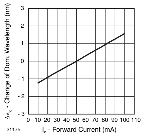
Fig. 7 - Change of Dominant Wavelength vs. Forward Current
