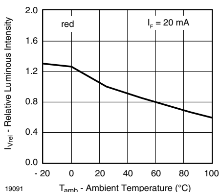
Fig. 30 - Relative Luminous Intensity vs. Ambient Temperature
