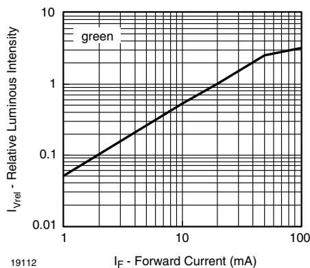
Fig. 23 - Relative Luminous Intensity vs. Forward Current
