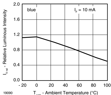
Fig. 10 - Relative Luminous Intensity vs. Ambient Temperature
