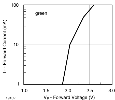
Fig. 22 - Forward Current vs. Forward Voltage
