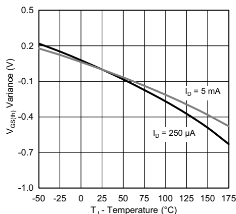
Threshold Voltage
