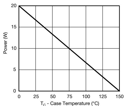
Power, Junction-to-Case
