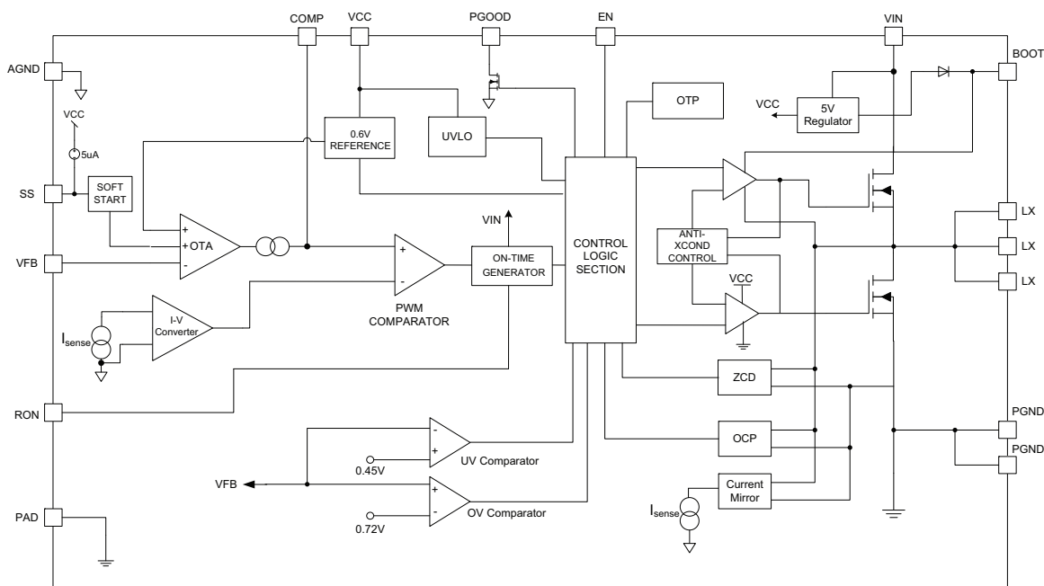
Fig. 2 - SiP12109 Functional Block Diagram
