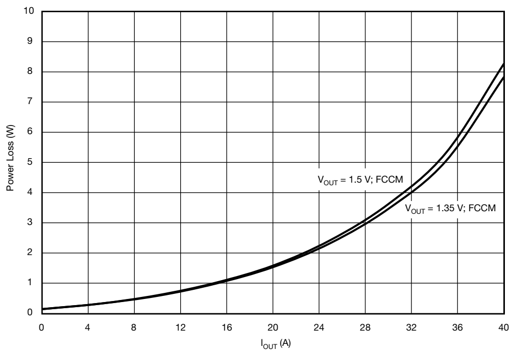
Fig. 7 - Power Losses vs. IOUT
