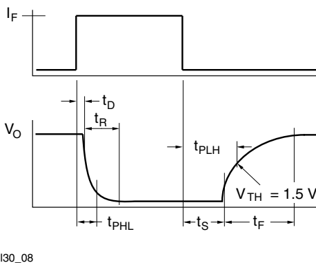
Fig. 8 - Switching Waveform
