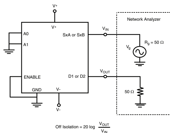
Fig. 7 - Off-Isolation
