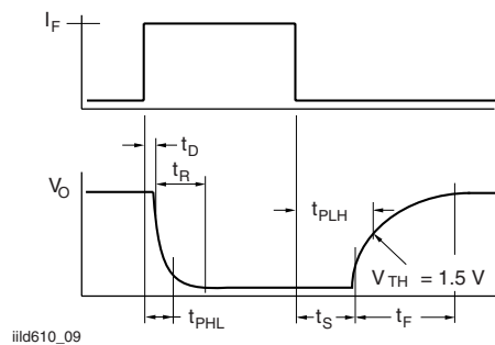
Fig. 9 - Switching Timing
