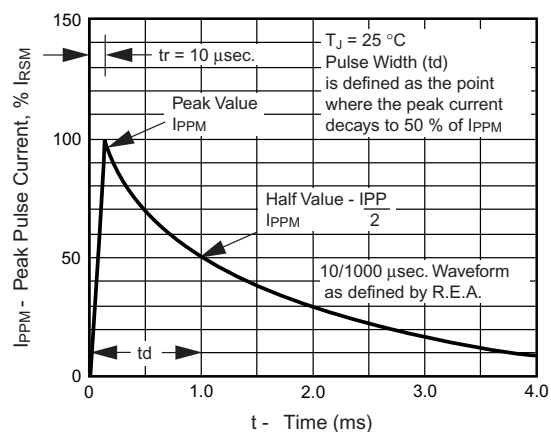
Figure 3. Pulse Waveform
