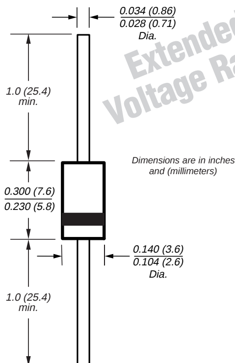
DO-204AC (DO-15)
