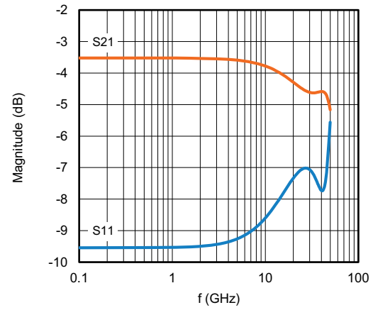
CH0603 wraparound ( Z_0 = Z_l = Z_s = R = 100 \Omega )
