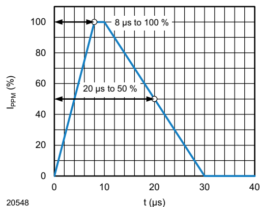
Fig. 2 - 8/20 µs Peak Pulse Current Wave Form acc. IEC 61000-4-5
