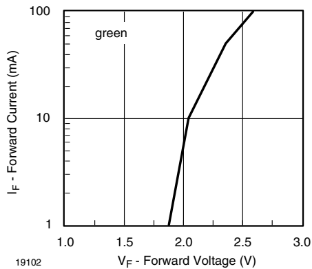
Fig. 15 - Forward Current vs. Forward Voltage
