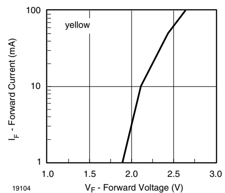
Fig. 20 - Forward Current vs. Forward Voltage
