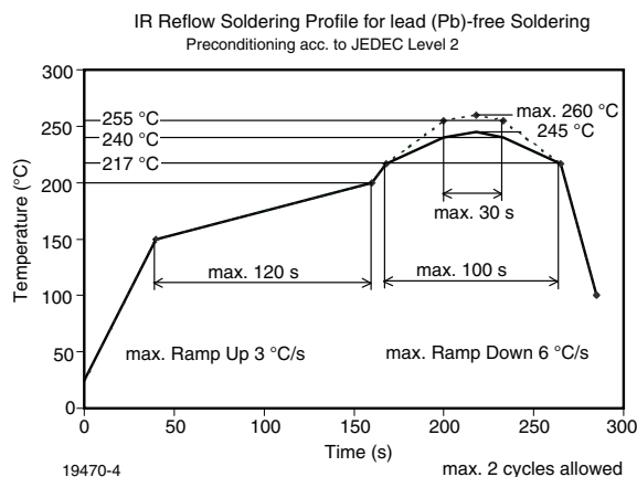
Fig. 27 - Vishay Lead (Pb)-free Reflow Soldering Profile (acc. to J-STD-020C)
