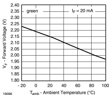
Fig. 14 - Forward Voltage vs. Ambient Temperature
