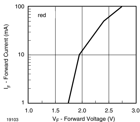
Fig. 25 - Forward Current vs. Forward Voltage
