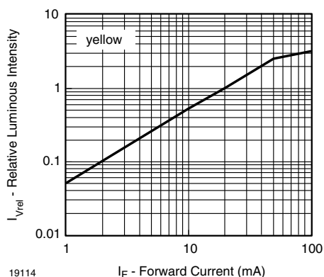
Fig. 21 - Relative Luminous Intensity vs. Forward Current
