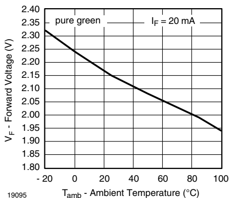
Fig. 9 - Forward Voltage vs. Ambient Temperature
