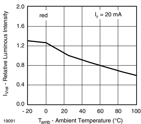
Fig. 23 - Relative Luminous Intensity vs. Ambient Temperature
