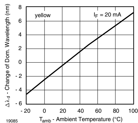
Fig. 17 - Change of Dominant Wavelength vs. Ambient Temperature
