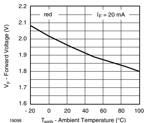
Fig. 24 - Forward Voltage vs. Ambient Temperature
