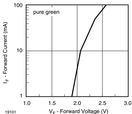
Fig. 10 - Forward Current vs. Forward Voltage
