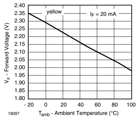
Fig. 19 - Forward Voltage vs. Ambient Temperature
