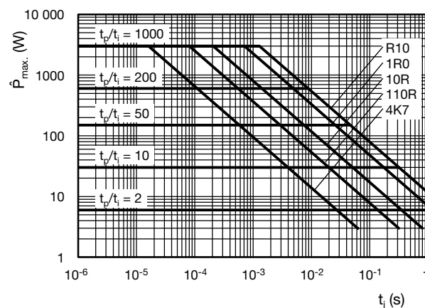
AC03 and AC03-AT Pulse on a regular basis; max. permissible peak pulse power ( P_{max} ) as a function of pulse duration ( t_i )
