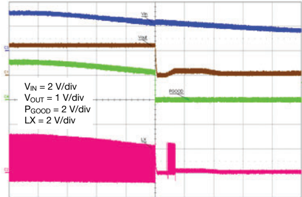
Shutdown PWM: 3 A Load
