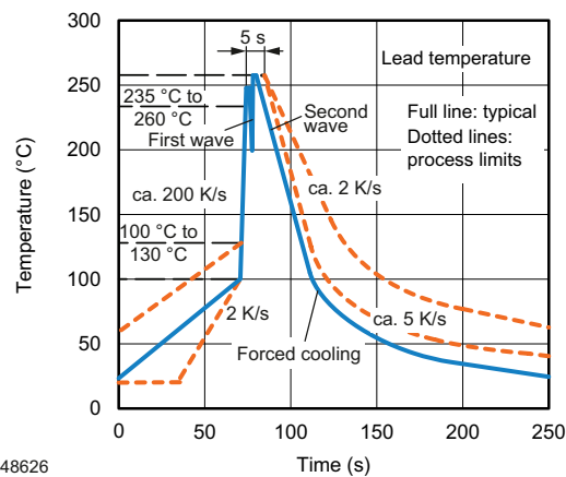
Fig. 15 - Wave Soldering Double Wave Profile According to J-STD-020 for DIP Devices
