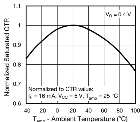
Fig. 13 - Normalized Saturated CTR vs. Ambient Temperature
