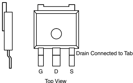
TO-252 Reverse Lead DPAK
