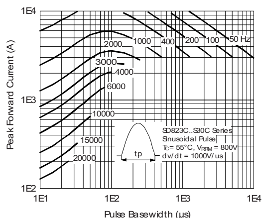
Fig. 39 - Frequency Characteristics
