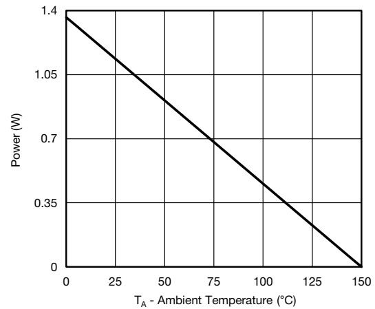
Power, Junction-to-Ambient
