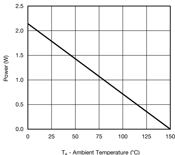
Power, Junction-to-Ambient
