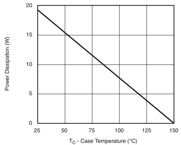
Power Derating
