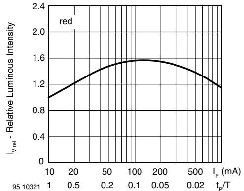
Figure 7. Rel. Luminous Intensity vs. Forw. Current/Duty Cycle
