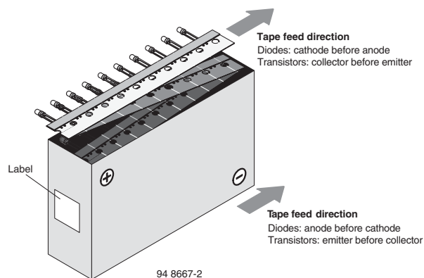
Figure 8. Tape Direction
