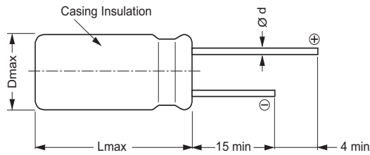
5 \leq \varnothing D \leq 18 Long leads EKB 00...
