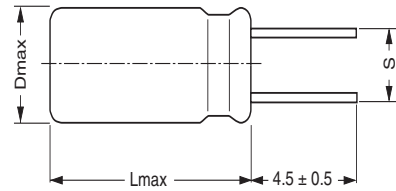
5 \leq \varnothing D \leq 18 Shortened leads EKB 05... (S = 2 / 2.5 / 3.5 / 5 / 7.5 mm)
