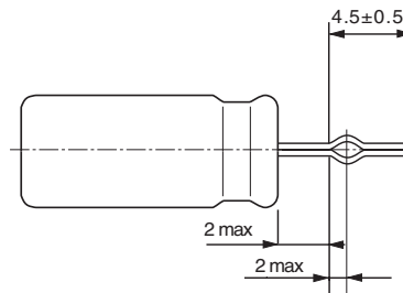
5 \leq \varnothing D \leq 8 Leads bent open, shortened and formed EKB 06... (S = 5 mm)
