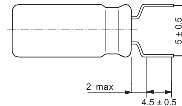
5 \leq \varnothing D \leq 8 Leads bent open, shortened EKB 09... (S = 5 mm)
