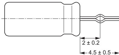
10 \leq \varnothing D \leq 18 Leads shortened and formed EKB 06... (S = 5 / 7.5 mm)
