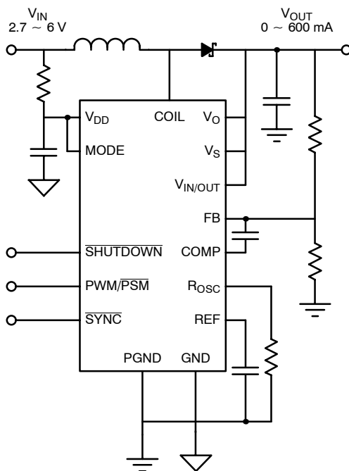
Boost Configuration
