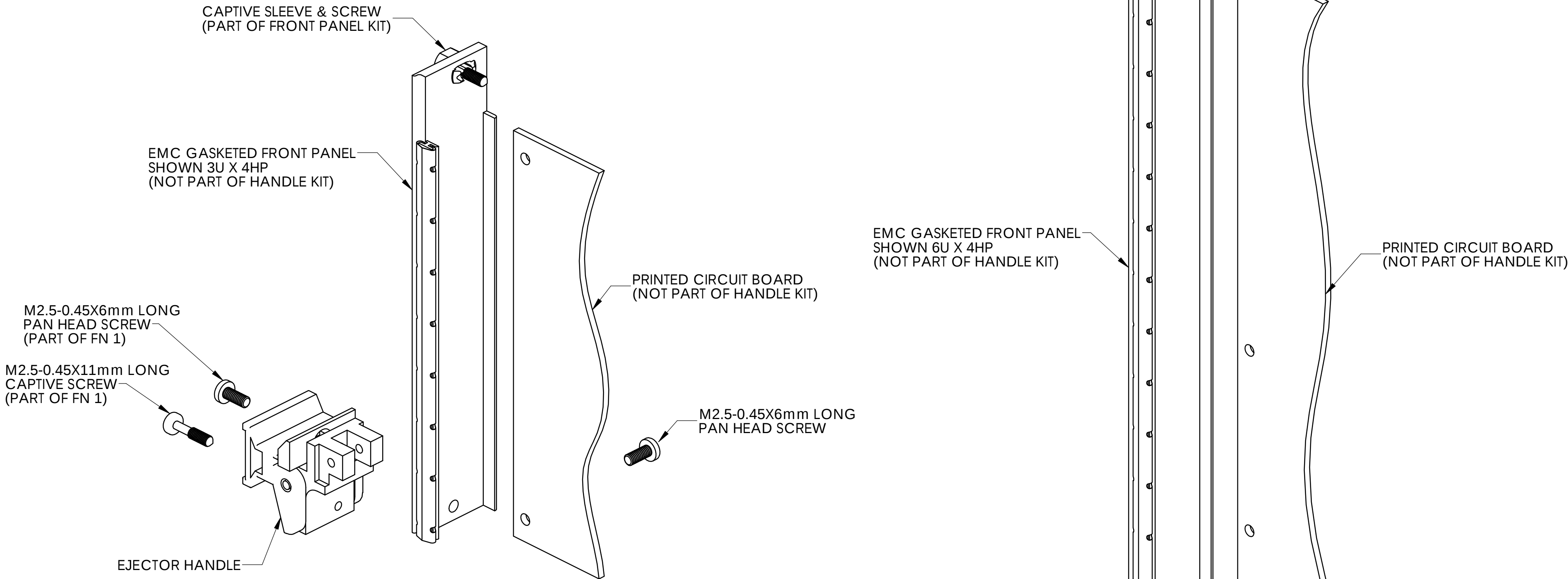
EXPLODED VIEW 3U PLUG-IN CARD ASSEMBLY
