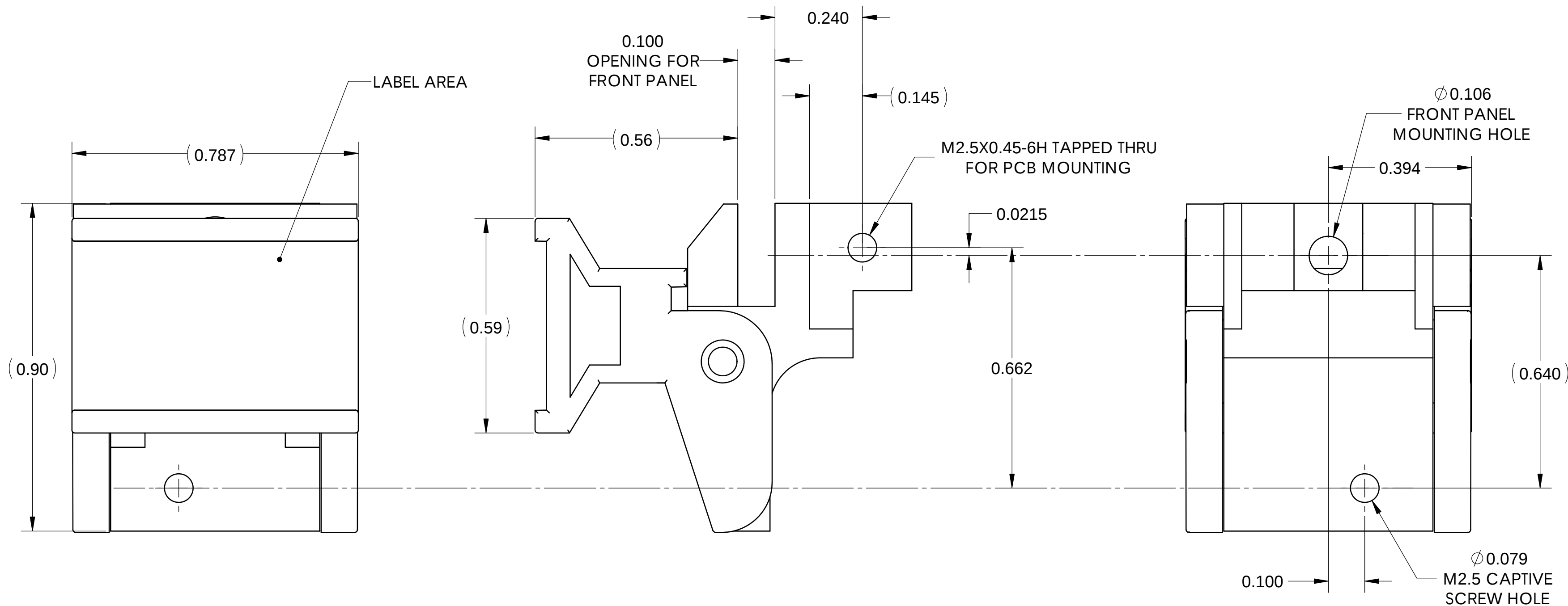
EJECTOR HANDLE DETAIL (HANDLE IS SYMMETRICAL FOR TOP OR BOTTOM INSTALLATION)
