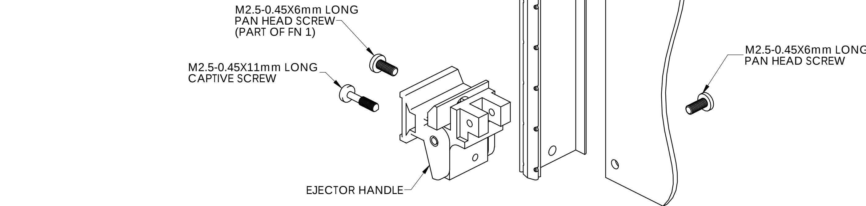
EXPLODED VIEW 6U OR 9U PLUG-IN CARD ASSEMBLY
