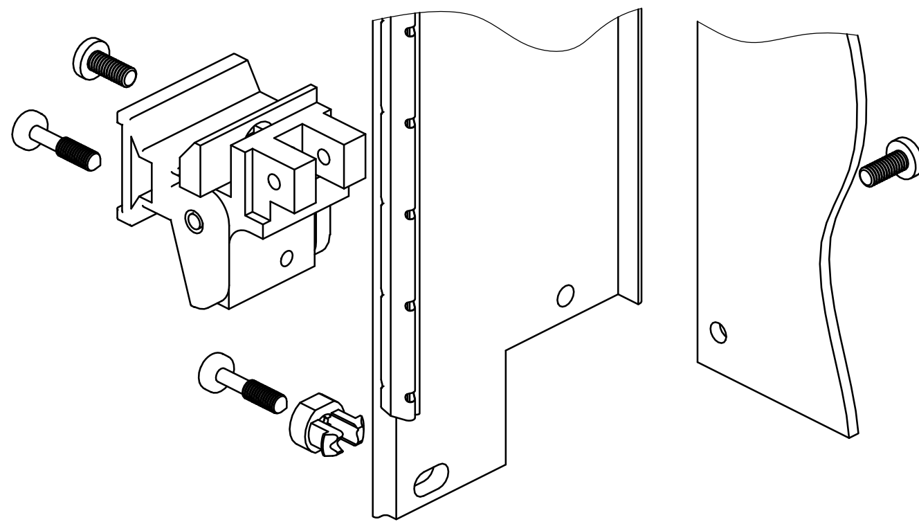
EXPLODED VIEW PANELS 8HP AND WIDER
