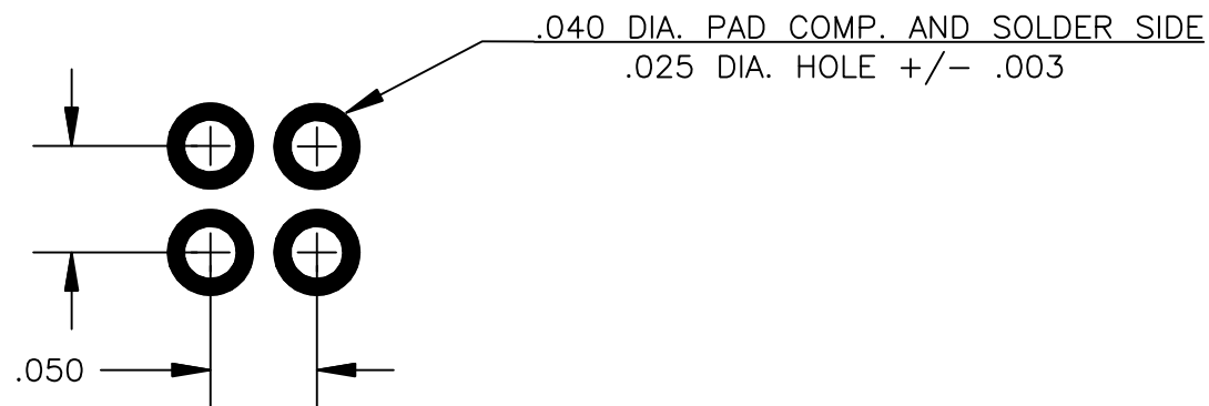
PATTERN DETAIL
