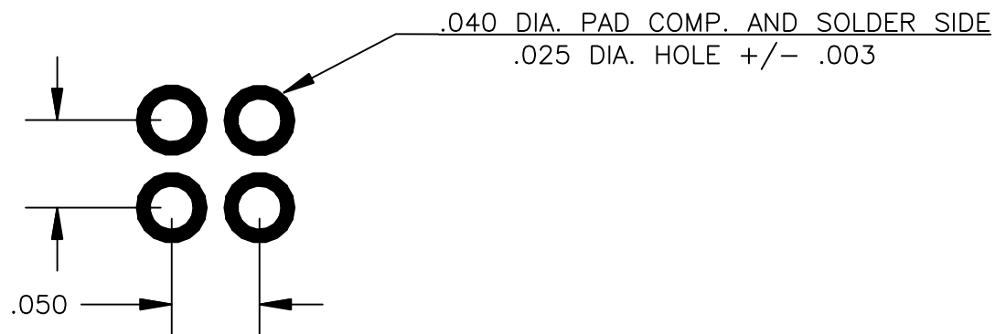
PATTERN DETAIL
