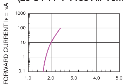
FORWARD VOLTAGE V_F (V) FORWARD CURRENT VS. FORWARD VOLTAGE
