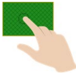
Figure 9-3: Tap Gesture.
