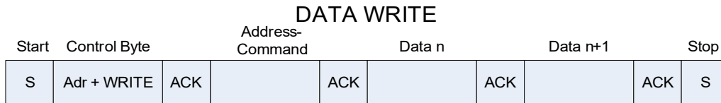
Figure 8.4 I2C Write
