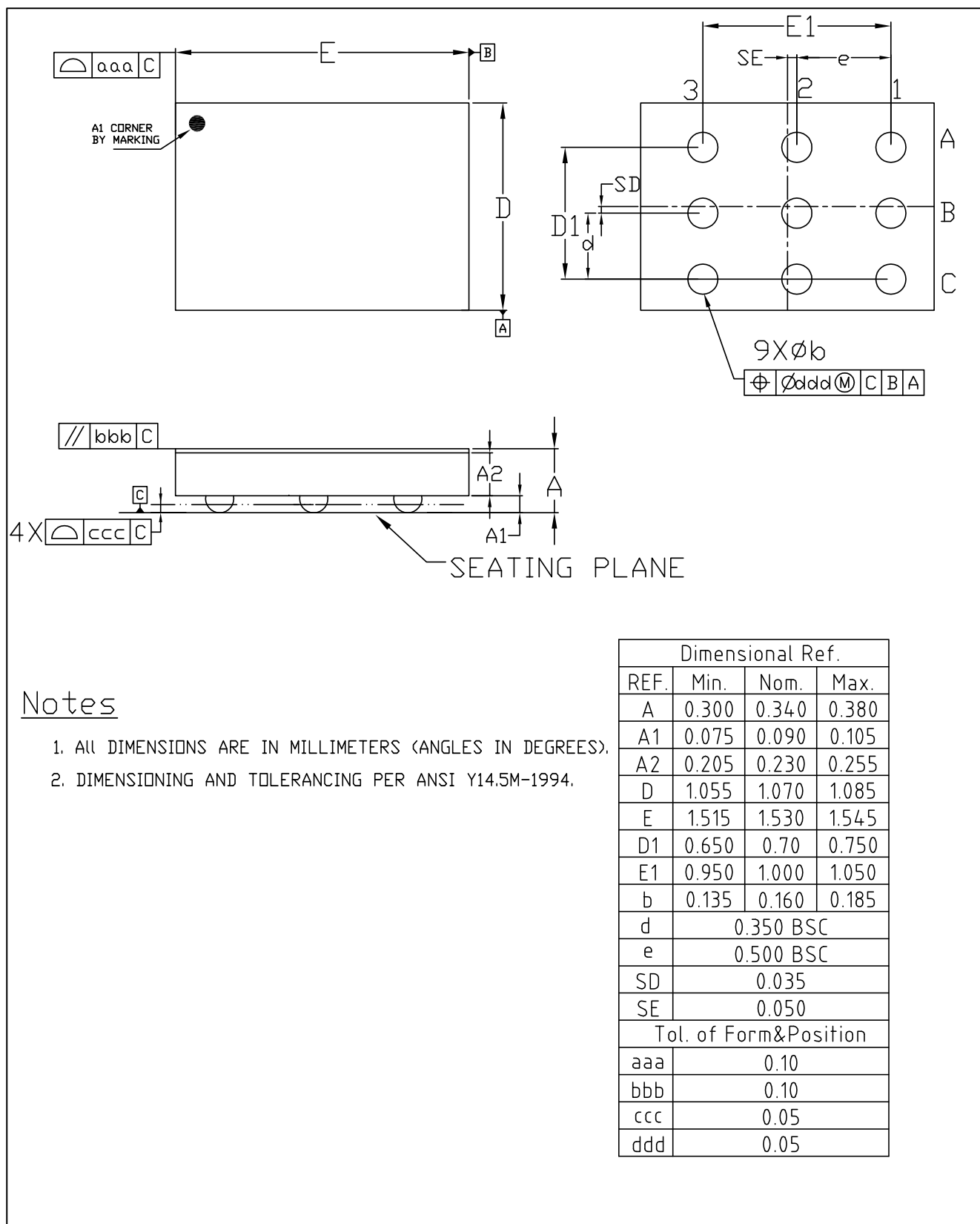
Figure 9-2 IQS624 WLCSP-9 package dimensions
