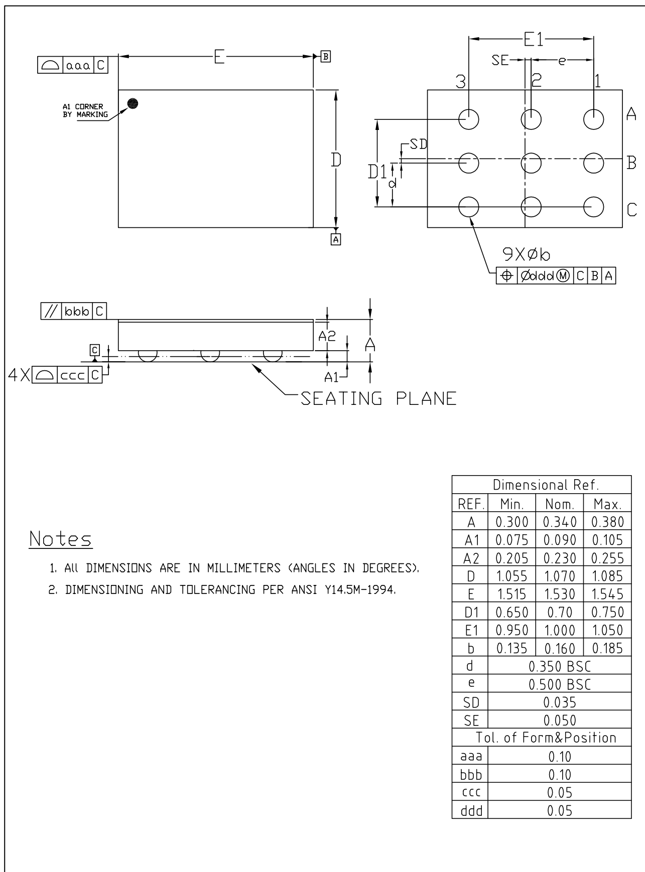
Figure 10.4 IQS620A WLCSP-9 package dimensions
