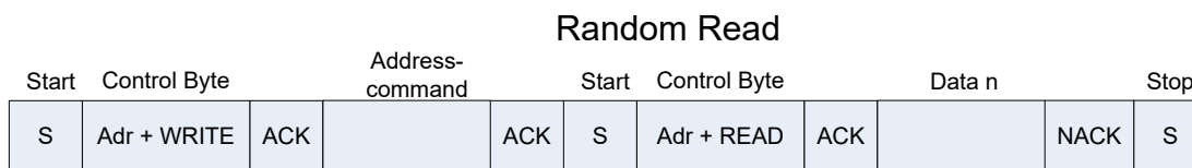
Figure 9.3 Random Read.
