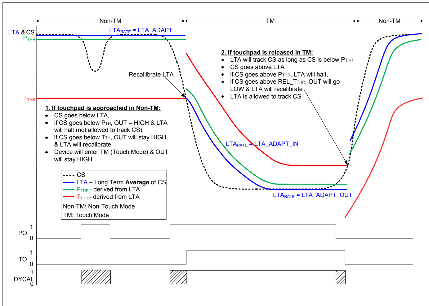
Figure 5.1: DYCAL Overview.
