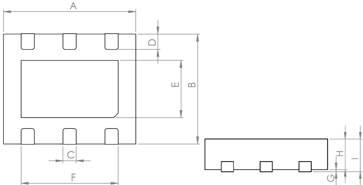
Figure 8.1 DFN-6 Packaging
