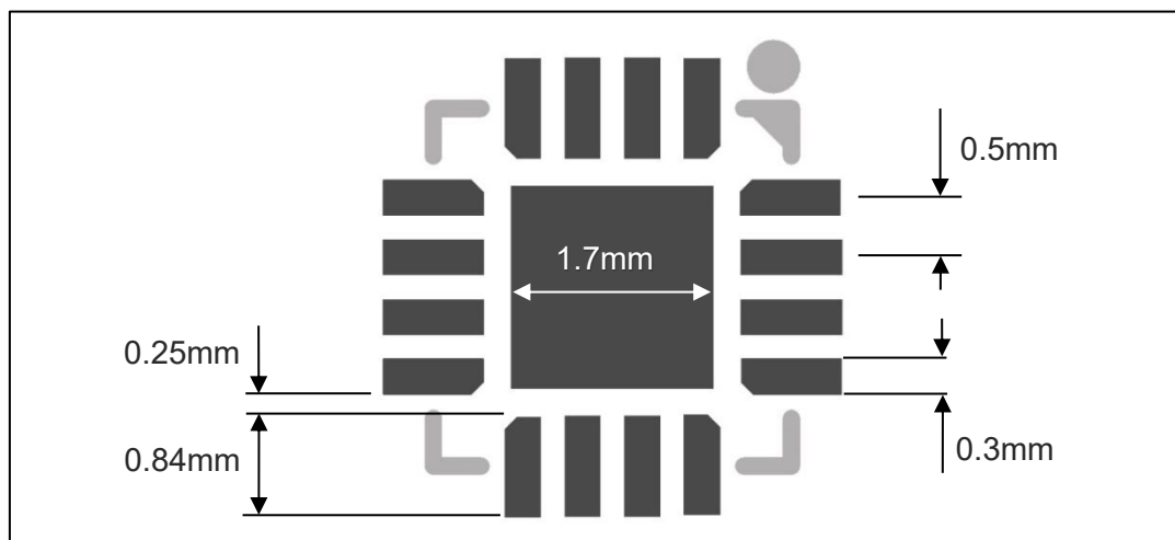
Figure 9.2 QFN-16 Footprint
