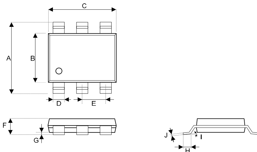
Figure 11.1 TSOT23-6 Packaging 6
