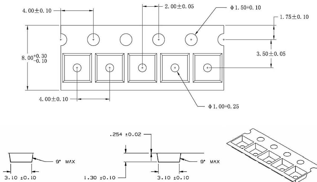
Figure 11.2 IQS128Tape Specification
