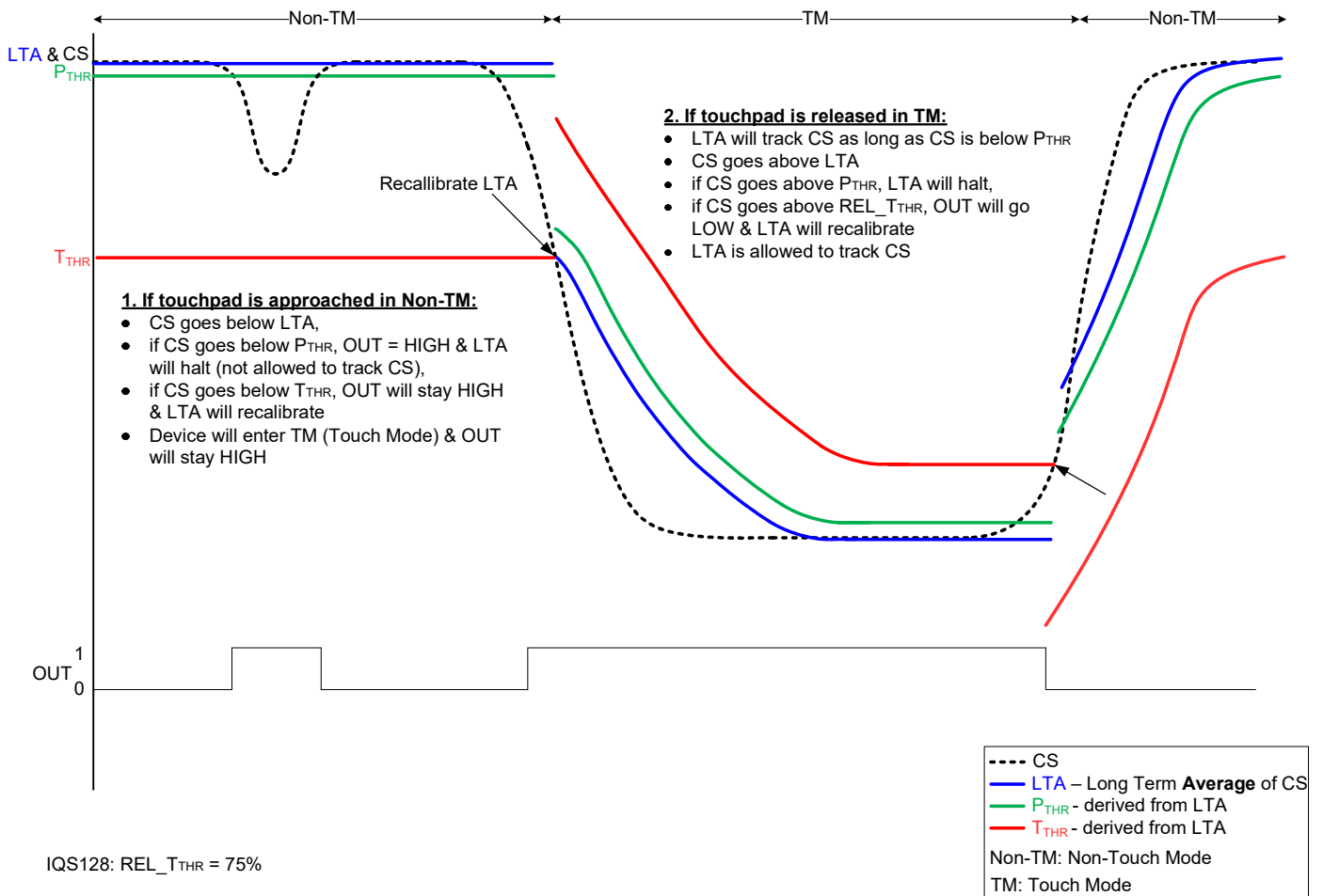
Figure 5.1 DYCAL Operation
