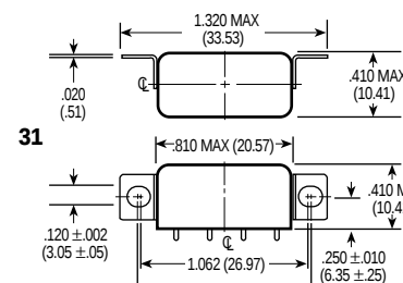
MOUNTING STYLES
