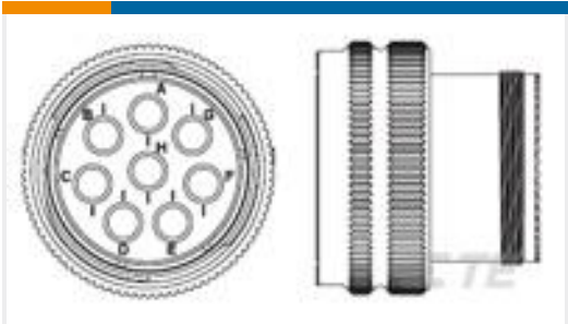
TE Part #1-1811928-4 8Q8 Size 25 Plug,A Key, OD
